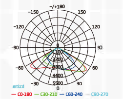
150W-Light Distribution Curve
