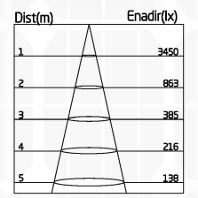
100W-Lux Distance Curve
