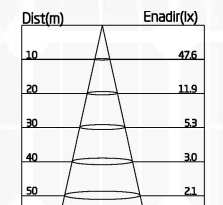
150W-Lux Distance Curve
