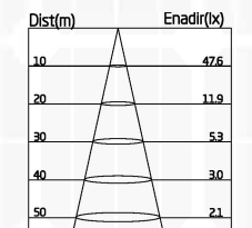
150W-Lux Distance Curve
