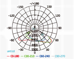
150W-Light Distribution Curve
