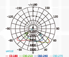
150W-Light Distribution Curve
