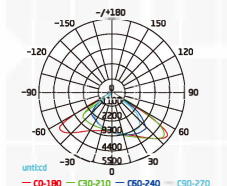
100W-Light Distribution Curve
