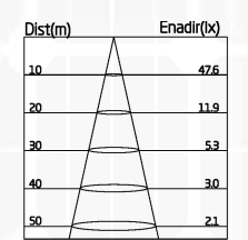
150W-Lux Distance Curve
