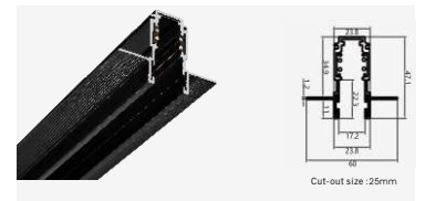
RH15-2A Size: L1000*W60*H47.1mm
