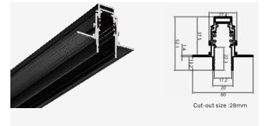
RH15-2S Size: L1000*W60*H52.1mm
