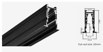
RH15-4 Size: L1000*W33.8*H56.3mm
