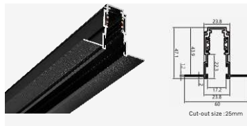
RH15-5 Size: L1000*W60*H47.1mm
