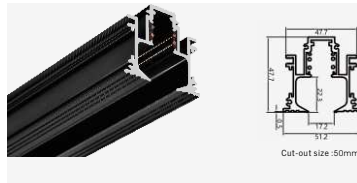
RH15-1 Size: L1000*W47.7*H47.7mm
